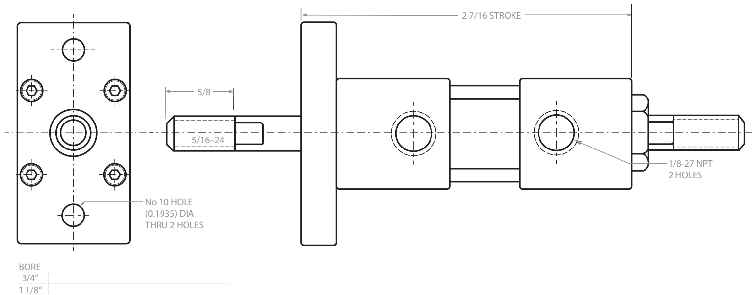
LITTLE AIR GIANT AIR CYLINDER · MODEL LG-DF · FLANGE MOUNTING
